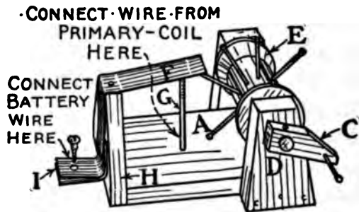
FIG. 194. — Interrupter for Shocking-Coil.
